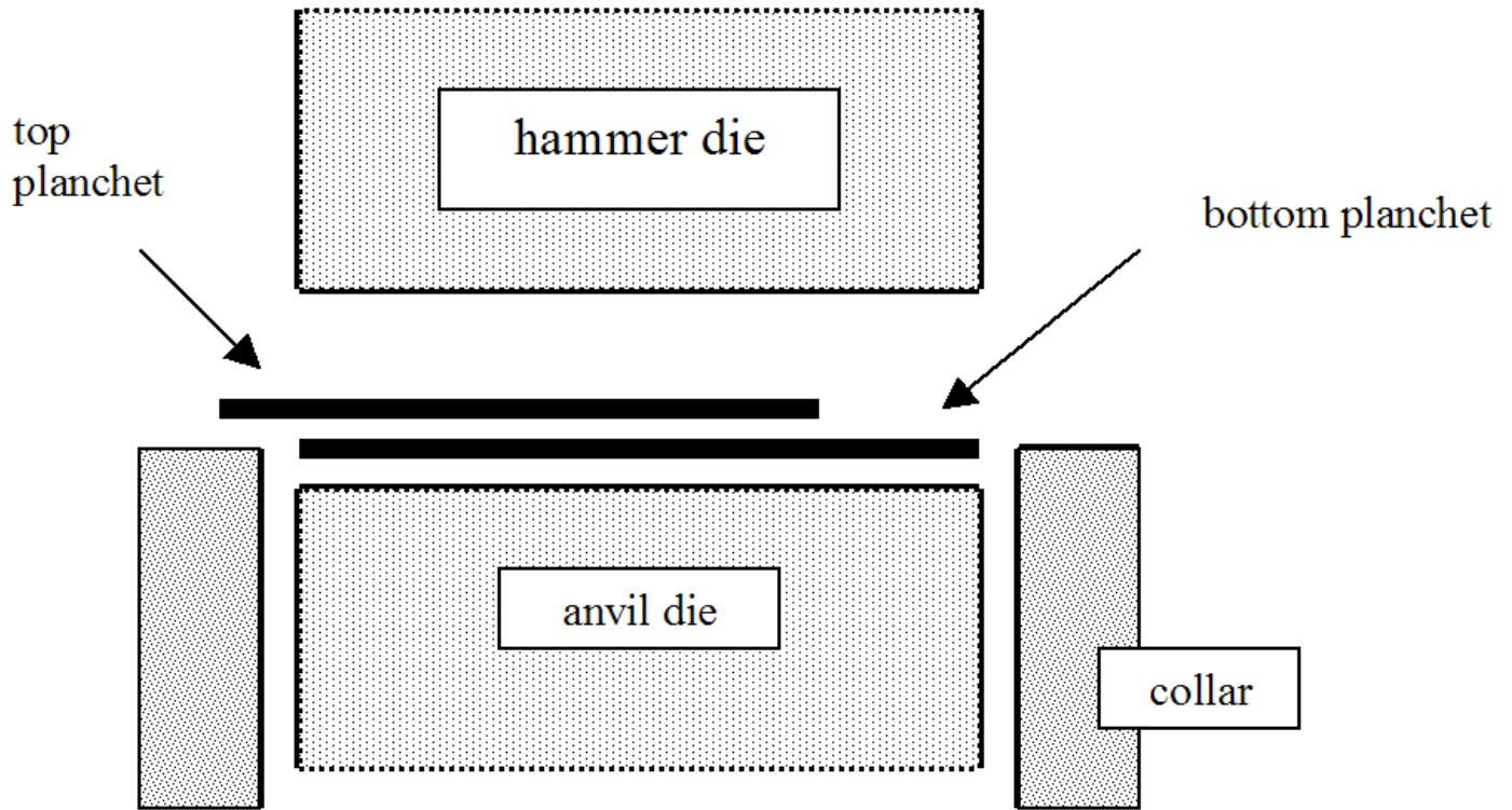
Figure 3a. Schematic diagram of a coinage press that will shortly produce an extrusion strike.
