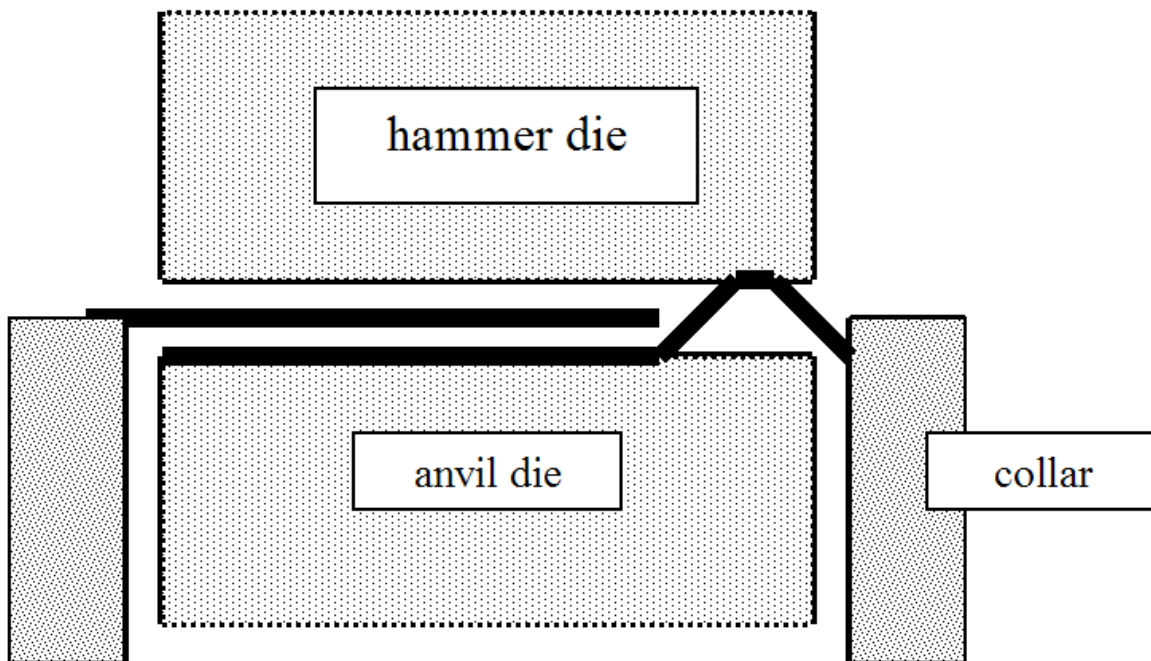
Figure 3b. Schematic diagram showing the aftermath of the strike. This is how the kind of extrusion strikes illustrated in this article form.
